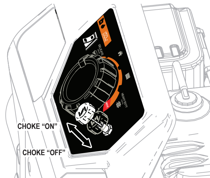
Figure 28 – Choke Knob
